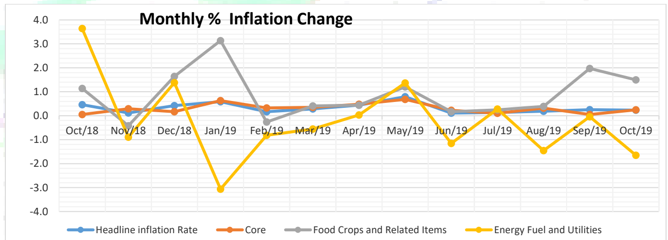
Graph 2: Somaliland Headline Monthly Inflation rates for 3 major components, October_2018-September_2019.
