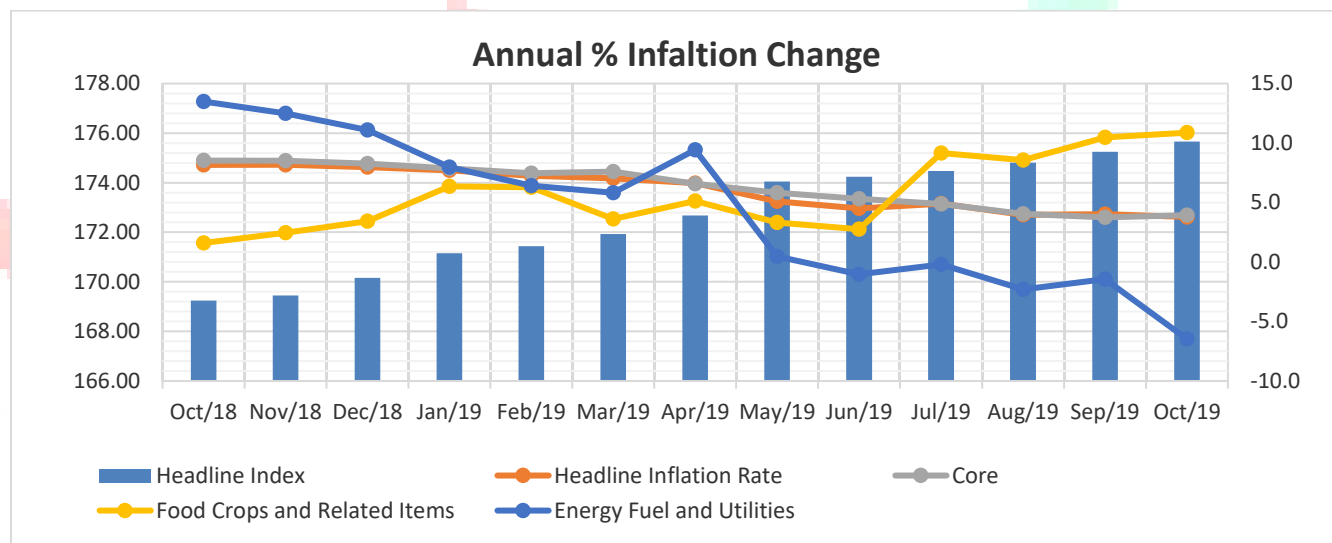
Graph 1: Somaliland Headline Index and Annual Inflation rates for 3 major components, October 2018 – October 2019: (2012 = 100)
